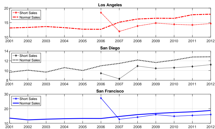
Figure B.29: Standard deviation of residuals from equation 2, respectively for short sales and normal sales, city by city; years from 2001 to 2012.
